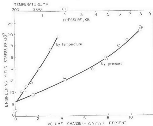
Cross-plot of engineering yield stresses against volume changes at the corresponding temperatures or pressures.
